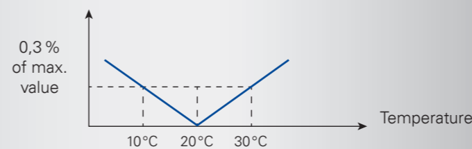
Temperature coefficient span
