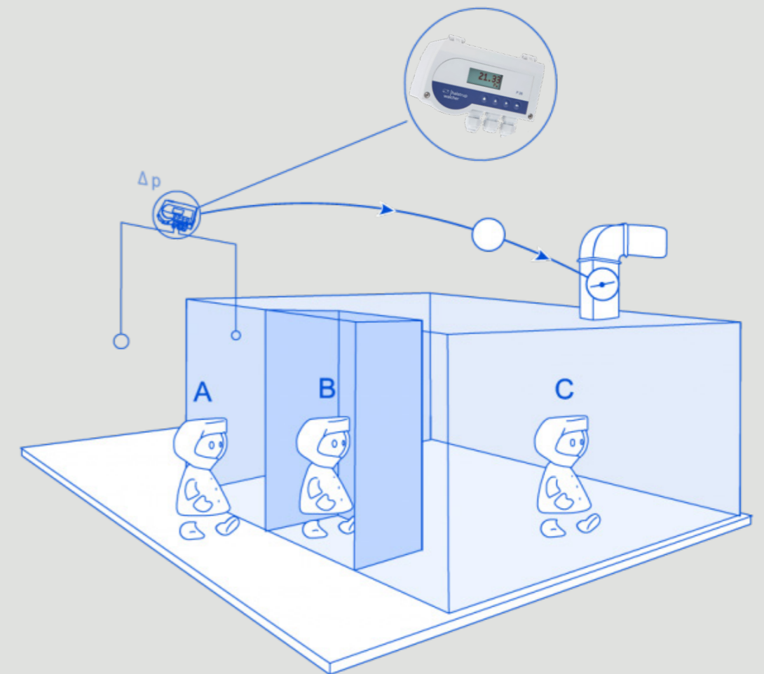
Pressure zone classification of a clean room with airlock
