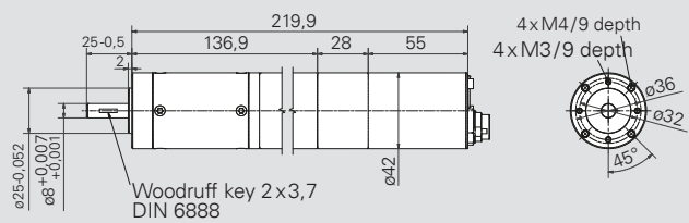
PSE 253-8-CA-M (with brake)
