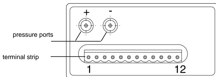
Fig. 5 rear view of the REG 21 pressure regulator
